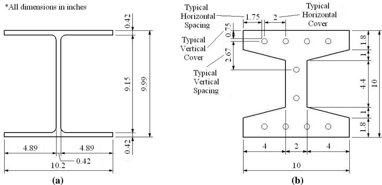
Figure 3.7. Dimensions of (a) an HP 10×57 steel pile and (b) a UHPC tapered H-shaped pile
