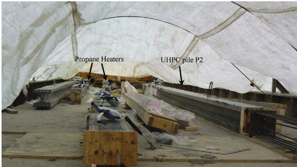
Figure 4.14. Stripped UHPC pile P2 undergoing initial curing with the help of propane heaters under tarp
